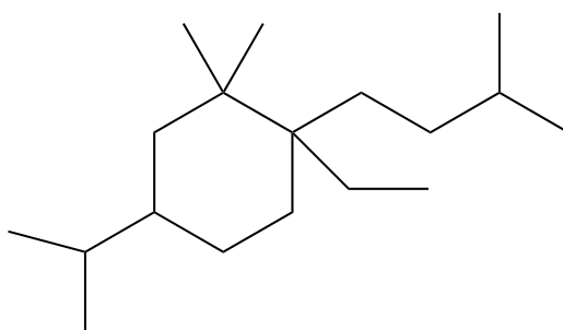
1-ethyl-1-isopentyl-4-isopropyl-2,2-dimethylcyclohexane
