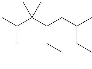
2,3,3,6-tetramethyl-4-propyloctane
