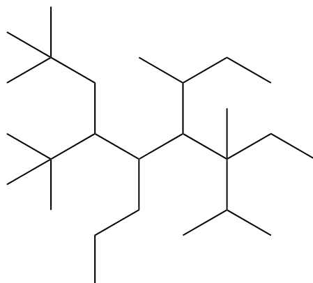
6-( sec -butyl)-4-( tert -butyl)-7-ethyl-2,2,7,8-tetramethyl-5-propylnonane
